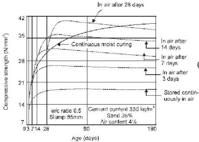
Fig. Development of Strength with Curing
