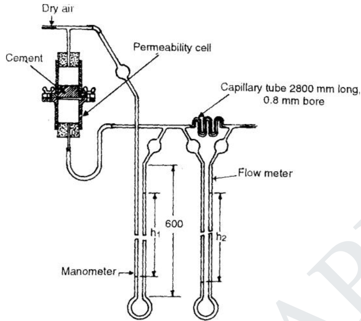
Fig. 28 Permeability Apparatus
