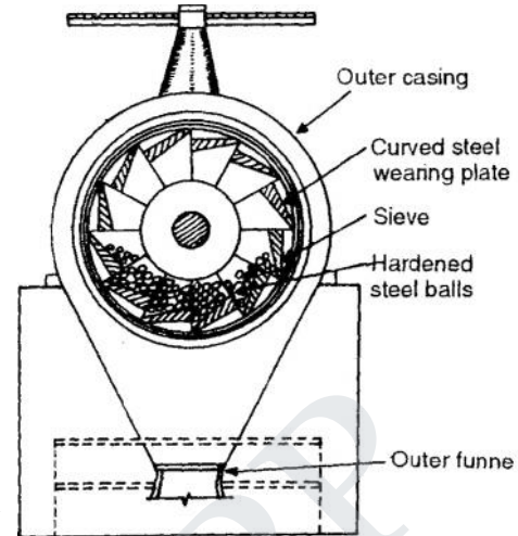
. 26 Ball Mill
