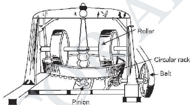
Fig. 19 Bullock Driven Mortar Mill (Ghanni)
