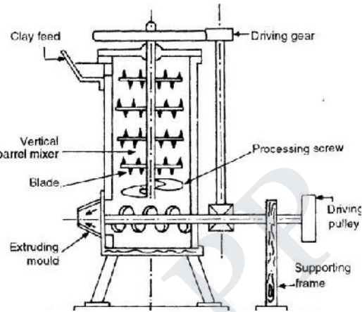
Fig 6 Pug Mill
