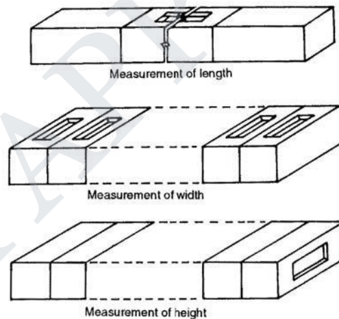
Fig. 16 Measurement of Tolerances of Common Building Bricks
