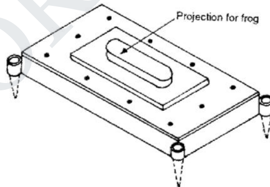
Fig. 9(b) Stock Board
