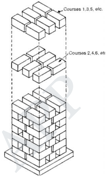
Fig. 11 Method of Drying Bricks
