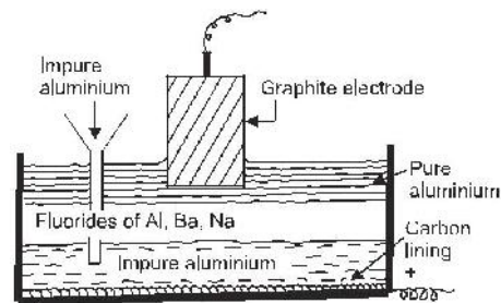
Fig. Hoop's Cell for Refining Aluminum
