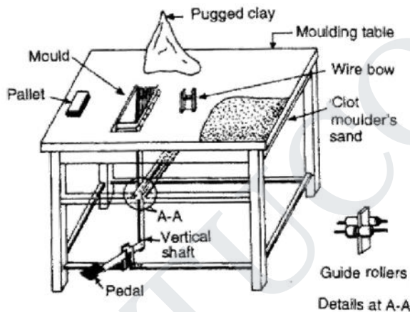
Fig. 9(a) Brick Moulding Table
