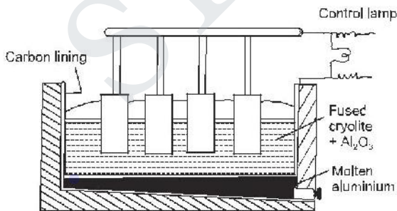
Fig. Extraction of Aluminum by Electrolysis
