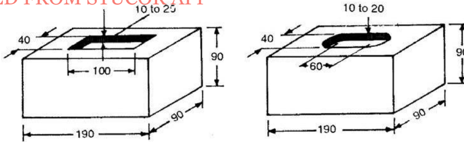
Fig. 5 Bricks with Frog
