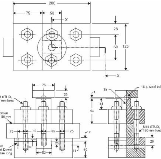
Fig. 3 Detail of Modified Johnson Shear Tool
