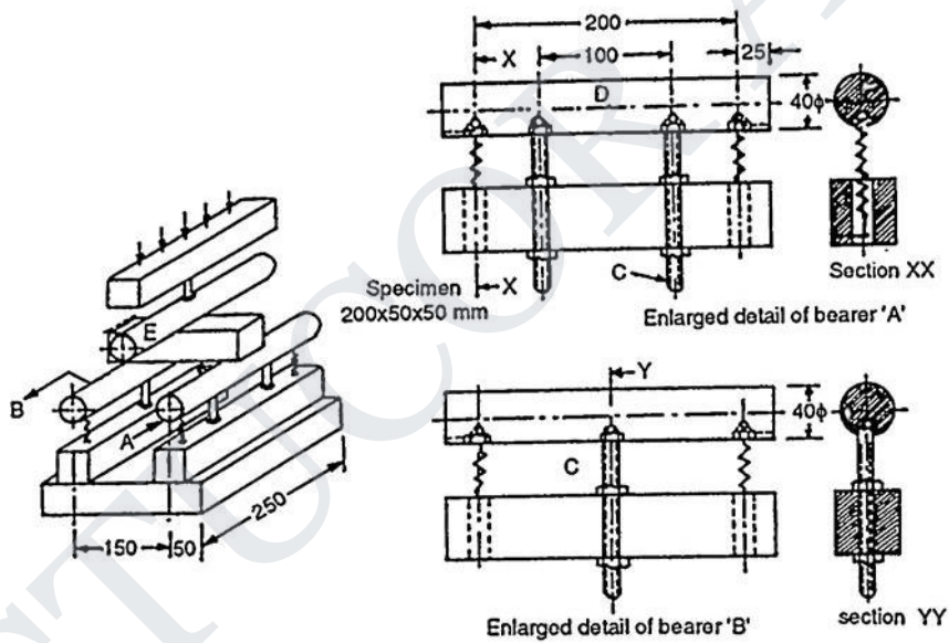
Fig. 1 Arrangement for Transverse Strength Test of Stones
