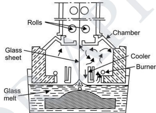
Fig. Machine for Vertical Drawing of Glass
