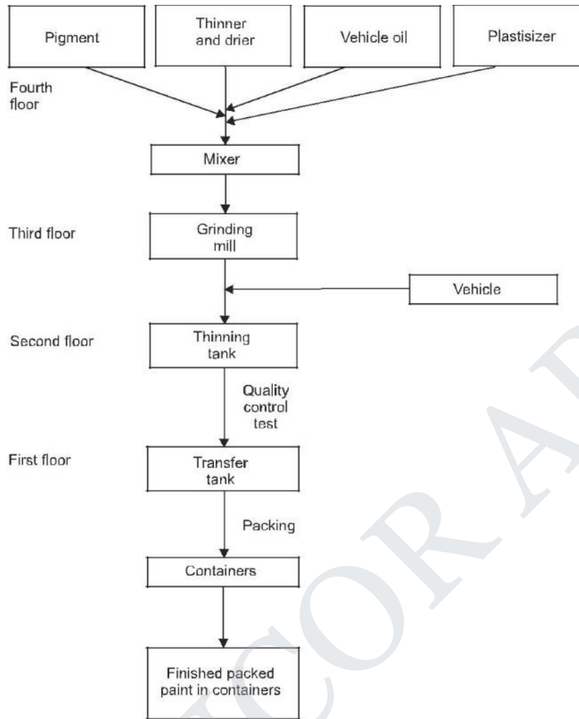
Fig. Flow Diagram of Paint Manufacture
