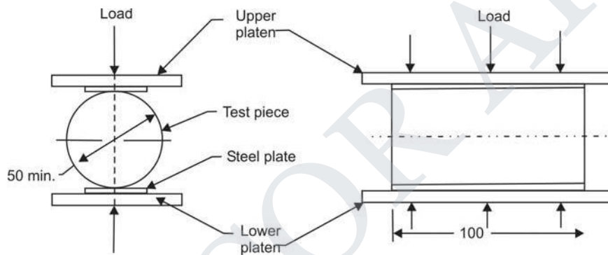
Fig. 2 General Arrangement for Testing Tensile Strength of Building Stone
