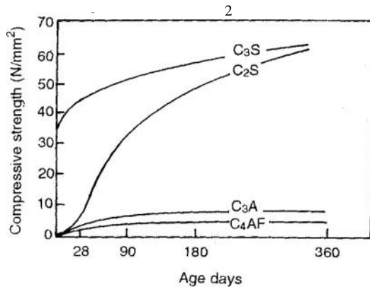
Fig. 21 Contribution of Cement Compounds to Strength of Cement
