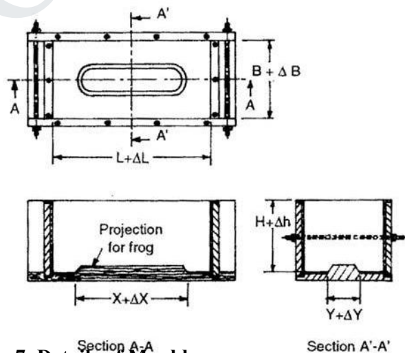
Fig 7. Details of Mould
