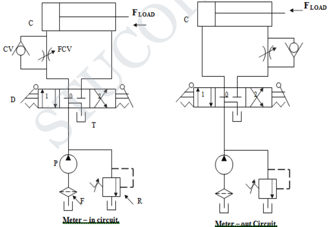
Meter – in Circuit
