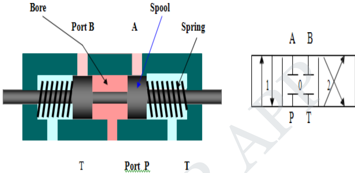
Mid Position: Closed Center 3 / 4 DCV
