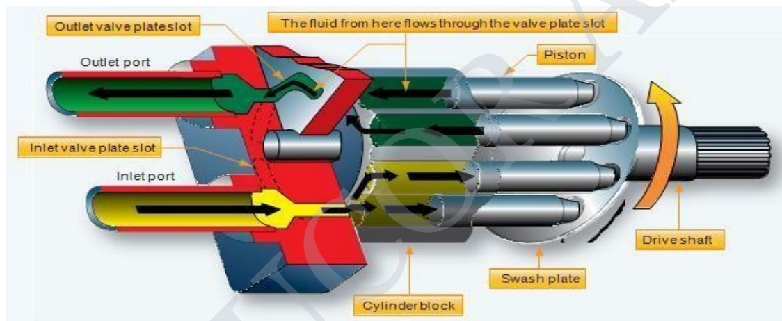
Fig. 2.1 Swash Plate Type
