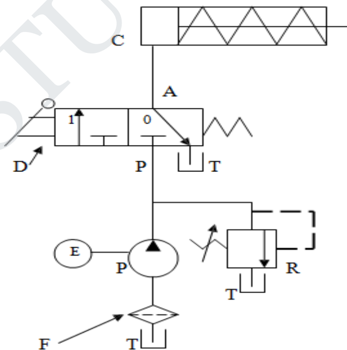
Figure shows a two-position, three way, manually operated, spring offset directional control valve ( DCV ) used to control the operation of a single – acting cylinder.
