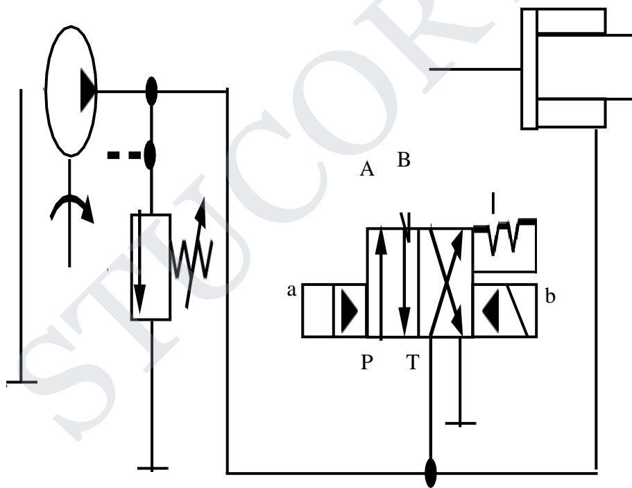
Regenerative Retraction Stroke
