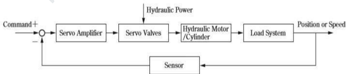
Fig. 9.1 Servo System Configuration
