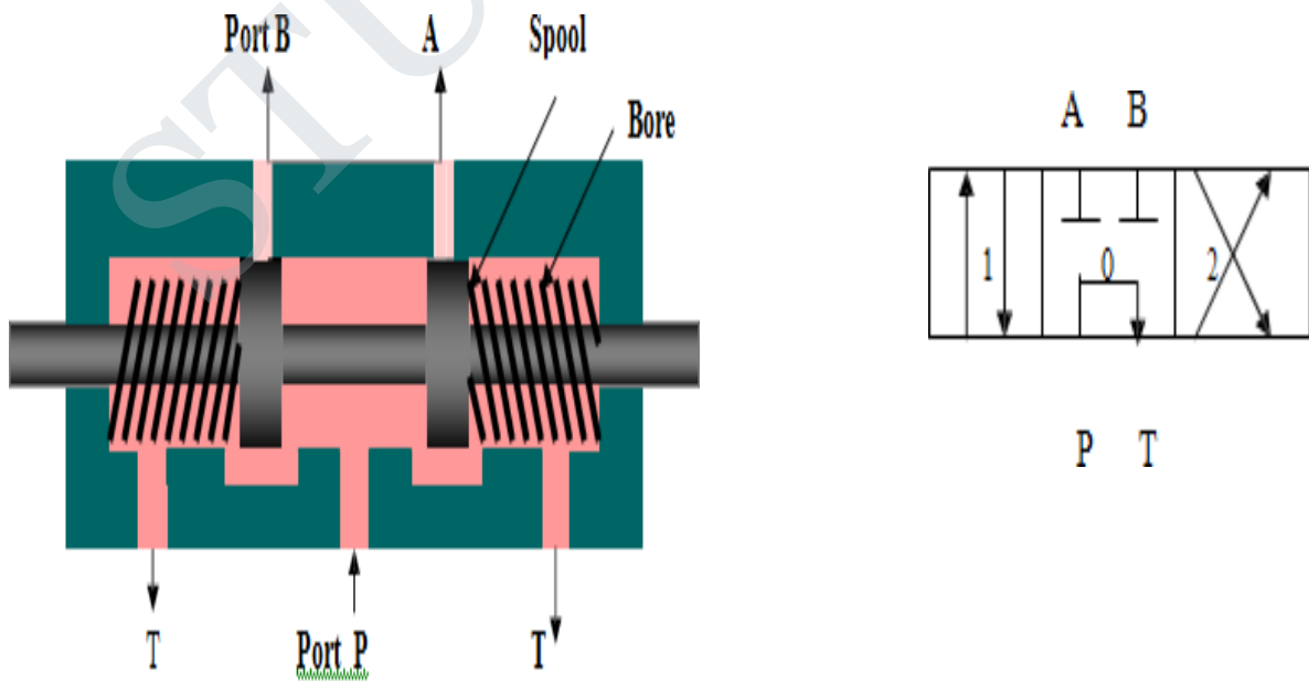
Tandem Center 3 / 4 DCV ; Mid position
